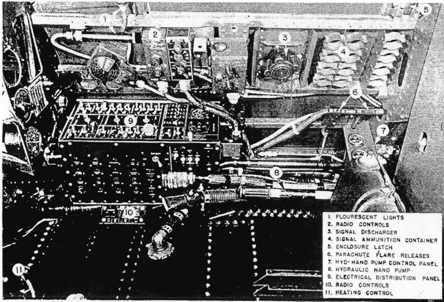
PILOT'S COCKPIT - RIGHT HAND SIDE
