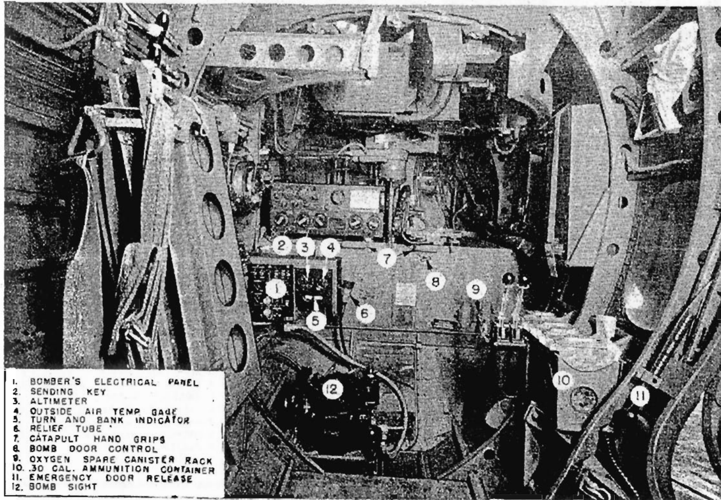
BOMBER COMPARTMENT - FORWARD
