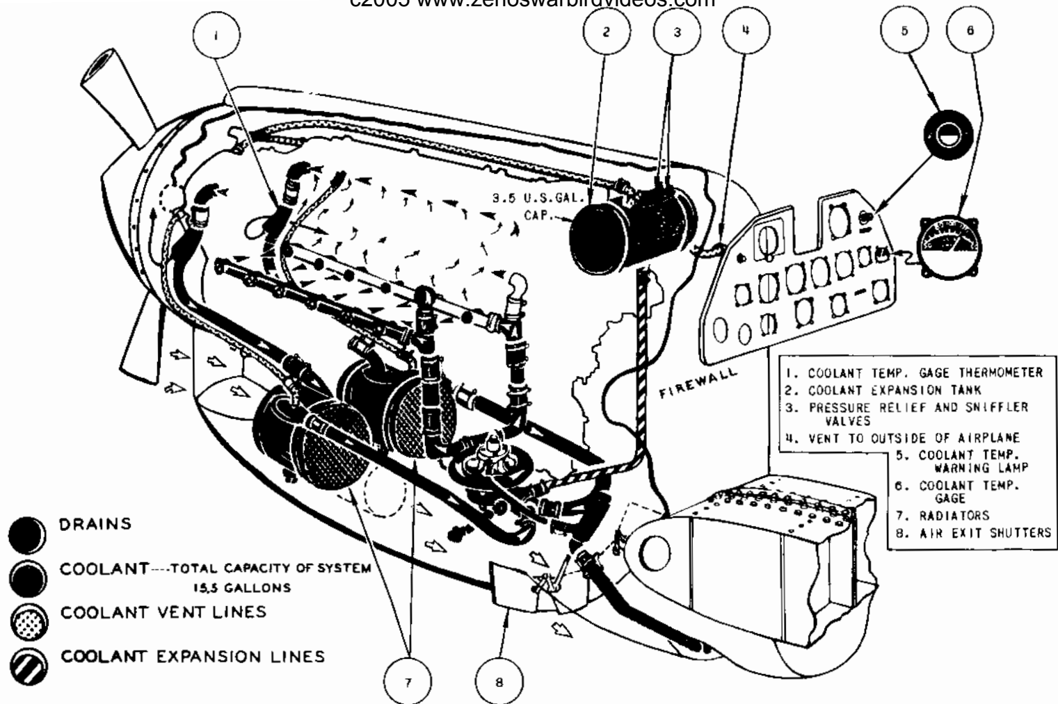
Figure 6 - Cooling System Diagram c2005 www.zenoswarbirdvideos.com
