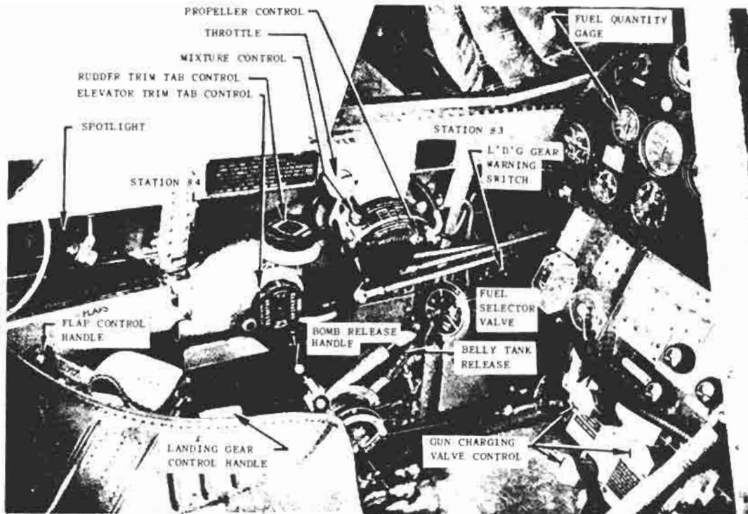
Figure 8 - Cockpit - Left Side c2005 www.zenoswarbirdvideos.com
