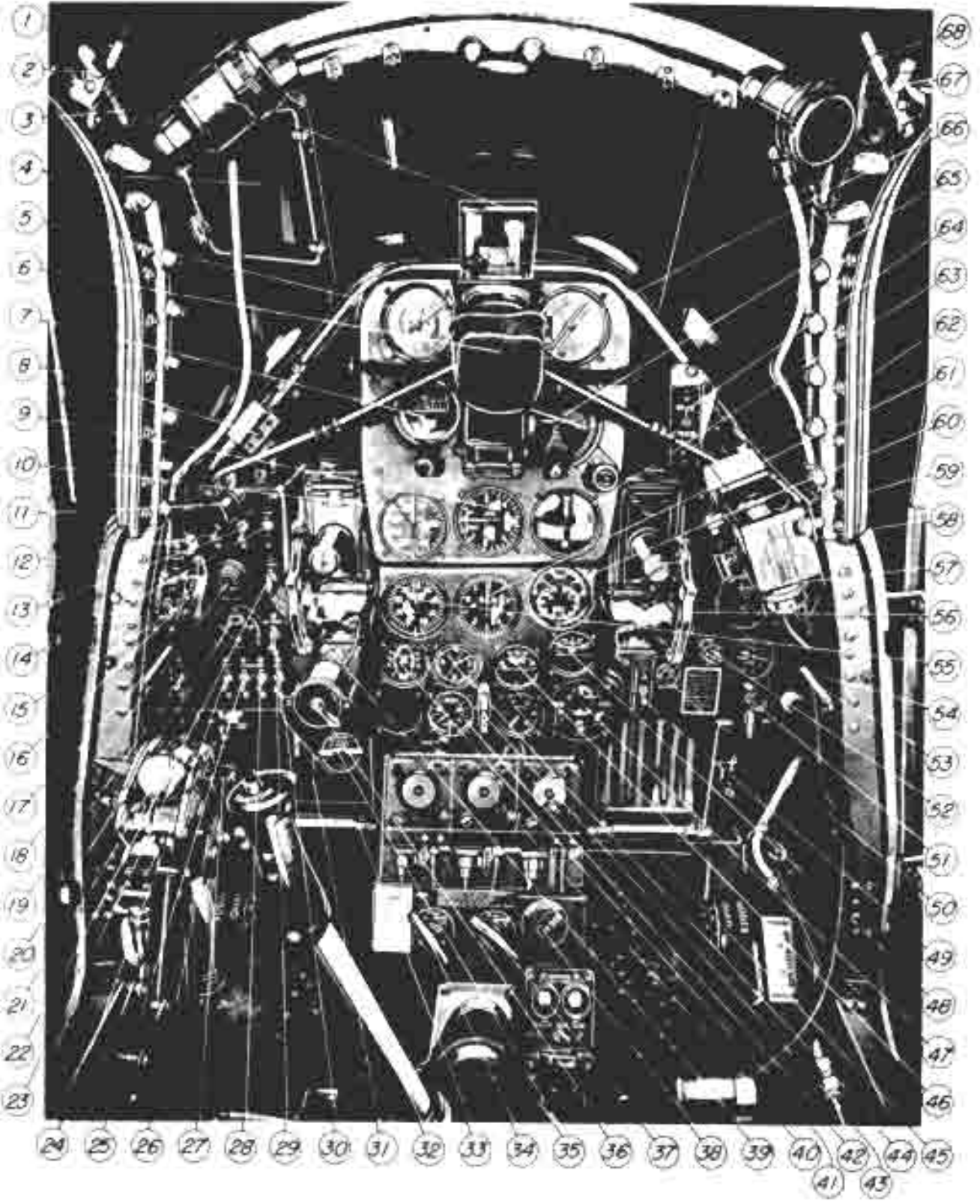
Figure 5 - Cockpit - Front View
