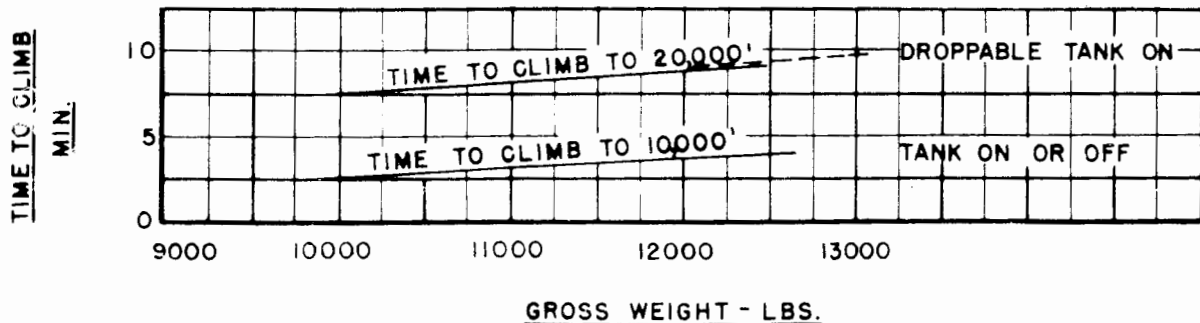
Figure 49 - Climb Chart
