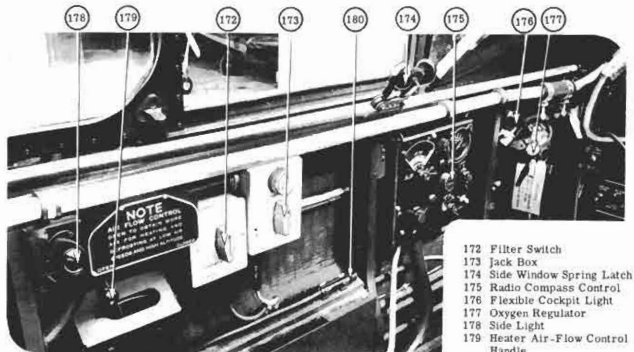
Figure 19 - Pilot's Compartment (Left Side)
