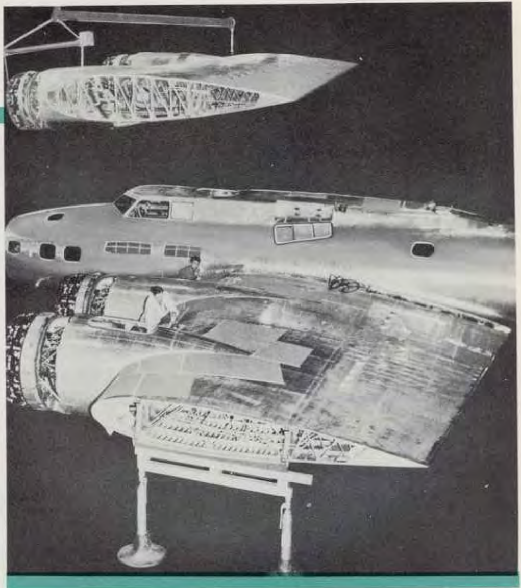
Figure 60— Nacelles Complete
