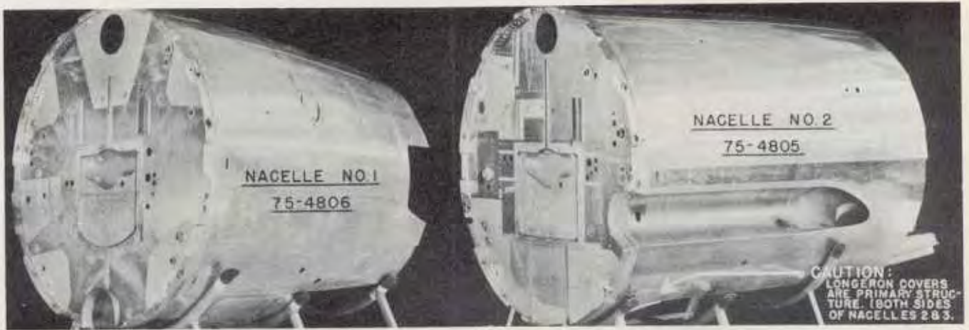
Figure 60— Nacelles Complete
