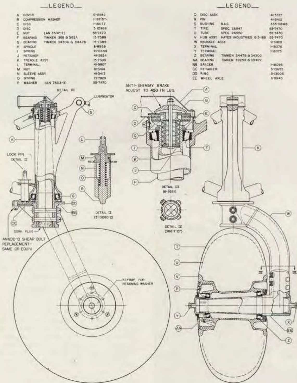
Figure 109—Tail Wheel Assembly Diagram (55-7470)
