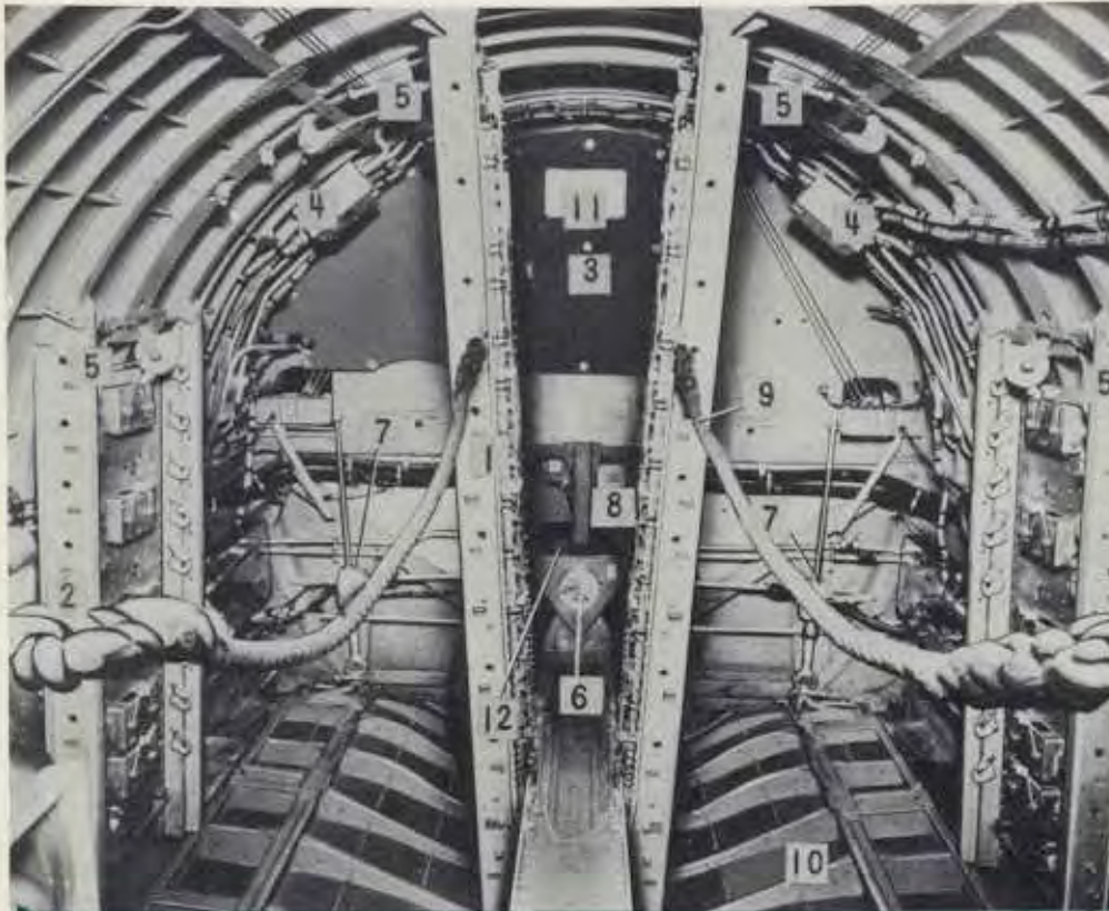
Figure 75—Bomb Bay (Fore and Aft)
