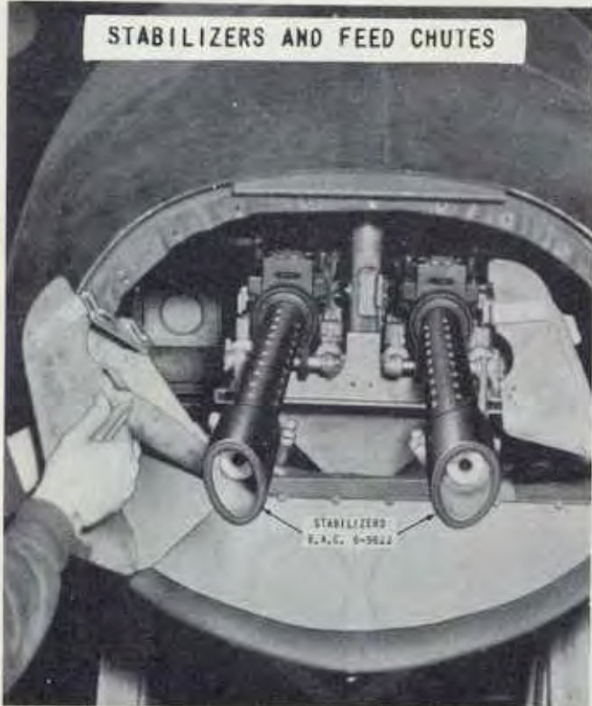
Figure 284B—Tail Gun Installation
