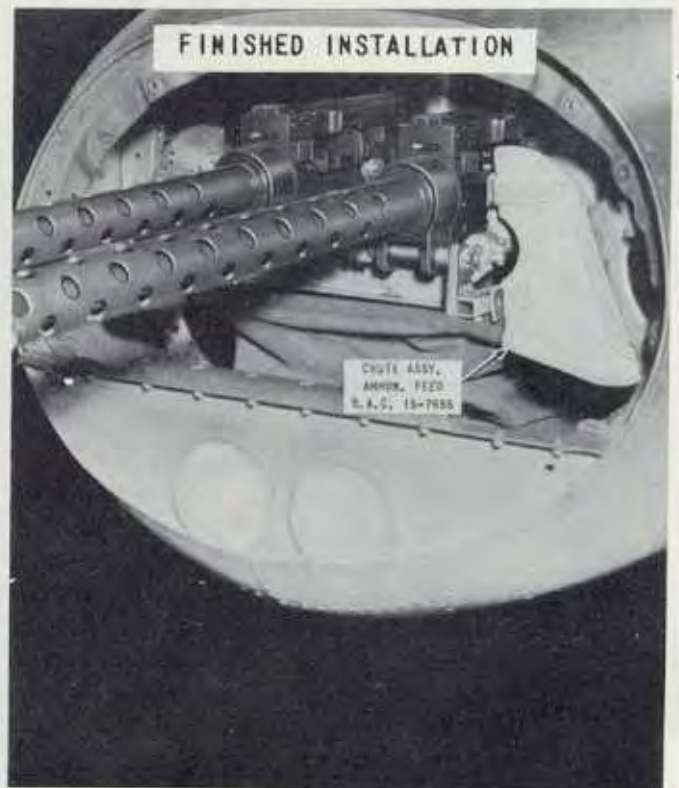
Figure 284B—Tail Gun Installation
