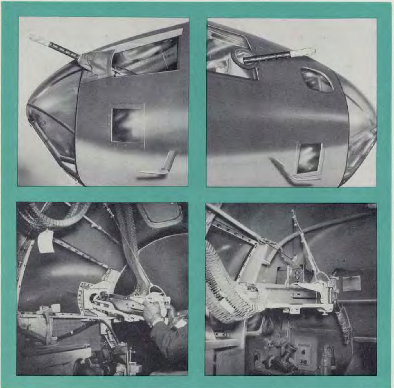
Figure 280—Nose Gun Installations
