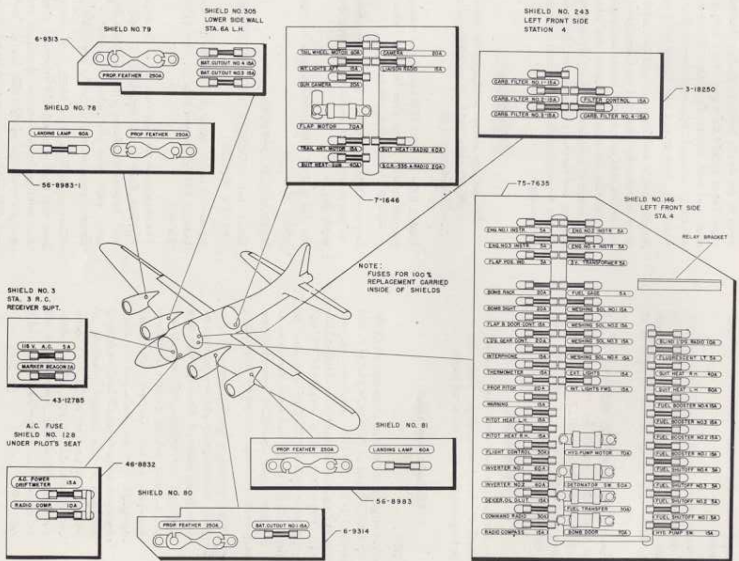
Figure 41 - Fuse Location Diagram
