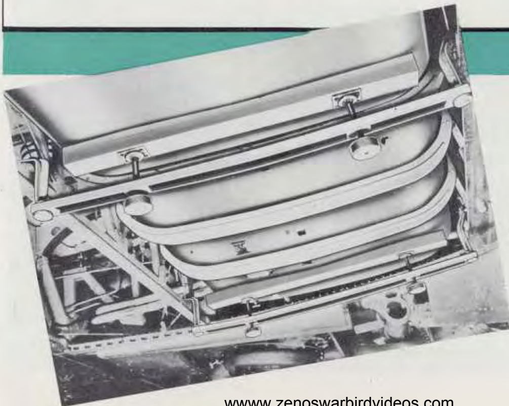
Figure 180—Typical Fuel Tank Installation Supports
