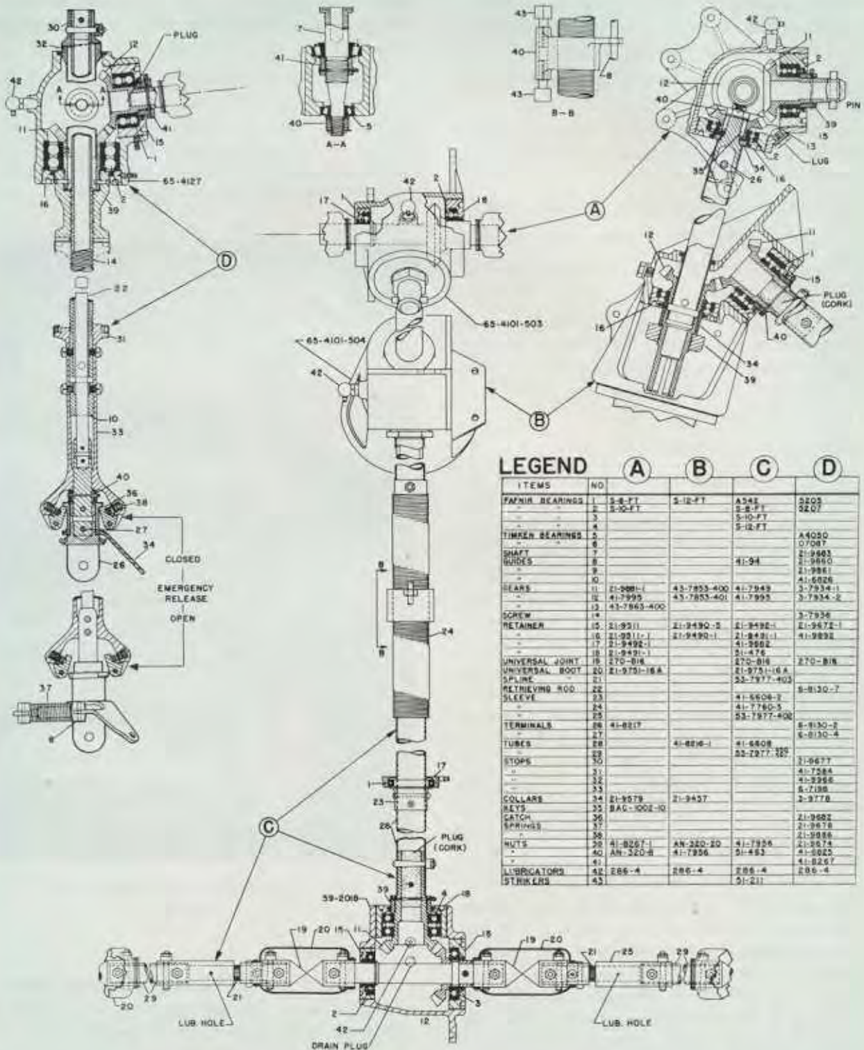
Figure 83—Bomb Bay Door Mechanism Details
