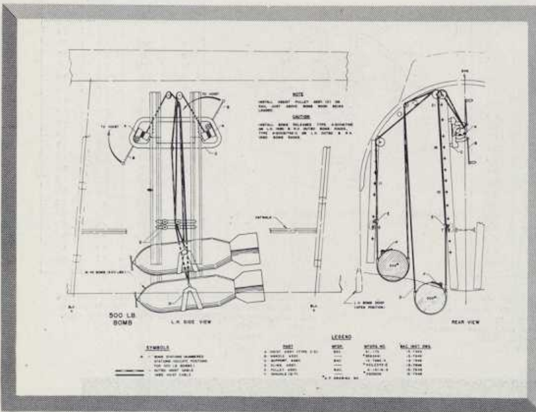
Figure 278B— Bomb Hoisting Diagram
