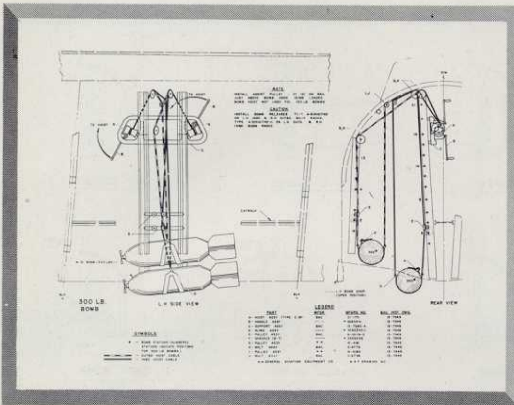
Figure 278A— Bomb Hoisting Diagram
