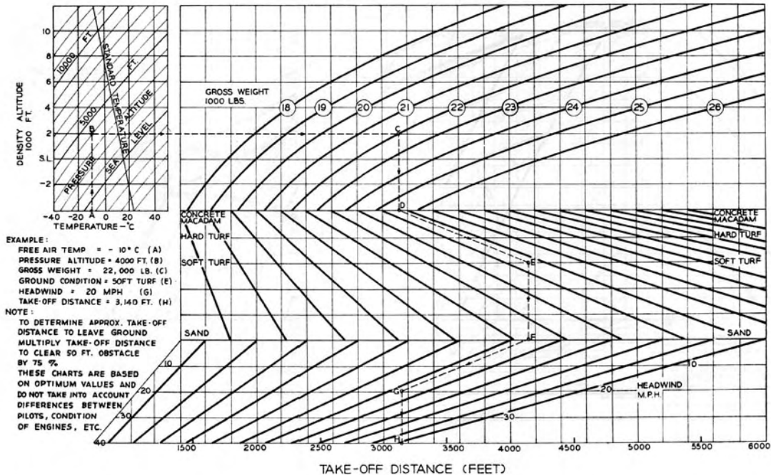
Figure 31—Take-Off Distance to Clear 50 ft Obstacle
