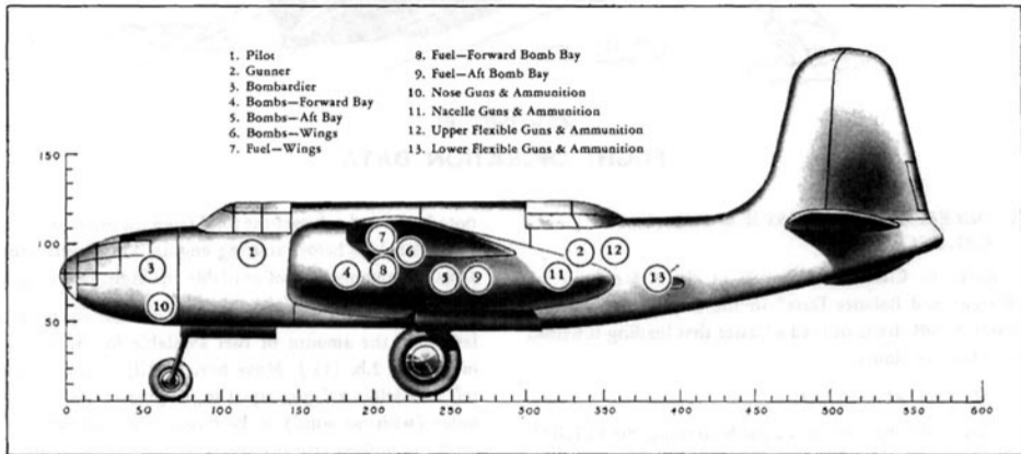
Figure 22—Stations Diagram
