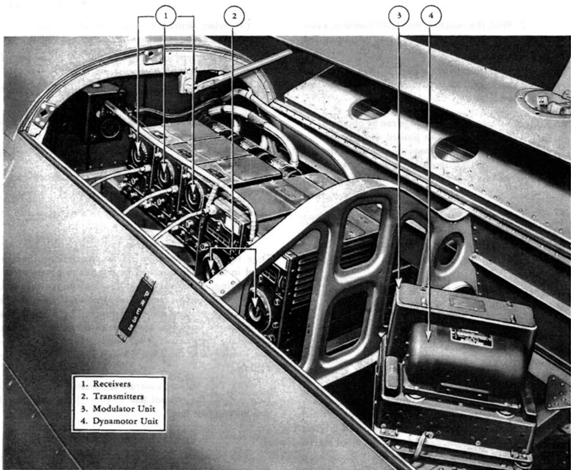
Figure 13—Communications Equipment in Fuselage
